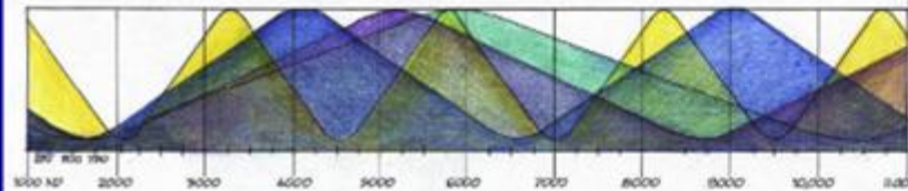
MONADIC RAY CYCLES
