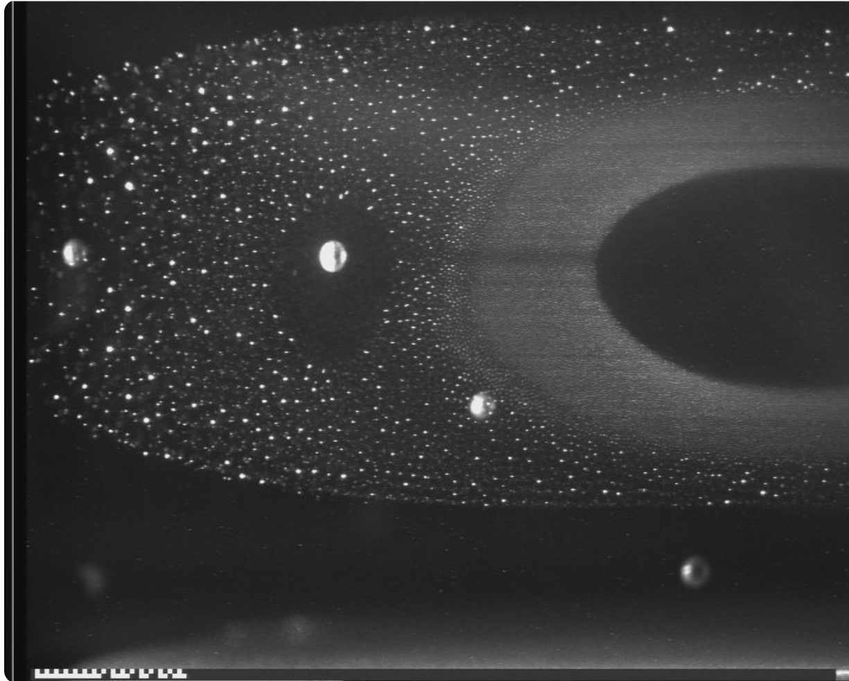
Dramatic end of plasma crystal experiment
