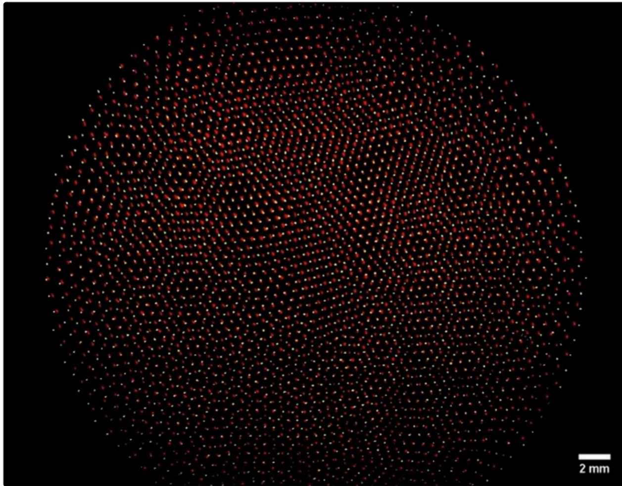
Frontiers | Preservation of a Dust Crystal as it Falls in an Afterglow Plasma
